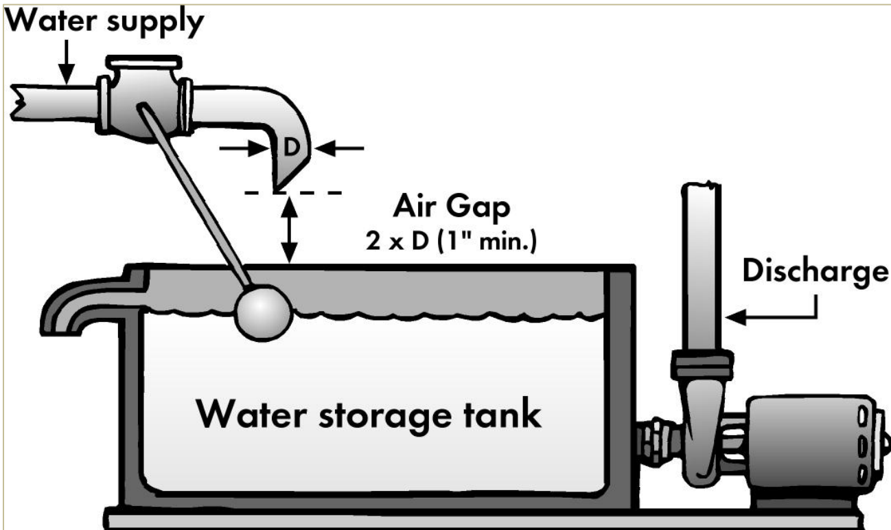
Air Gap backflow prevention configuration (usually used in greenhouses)
